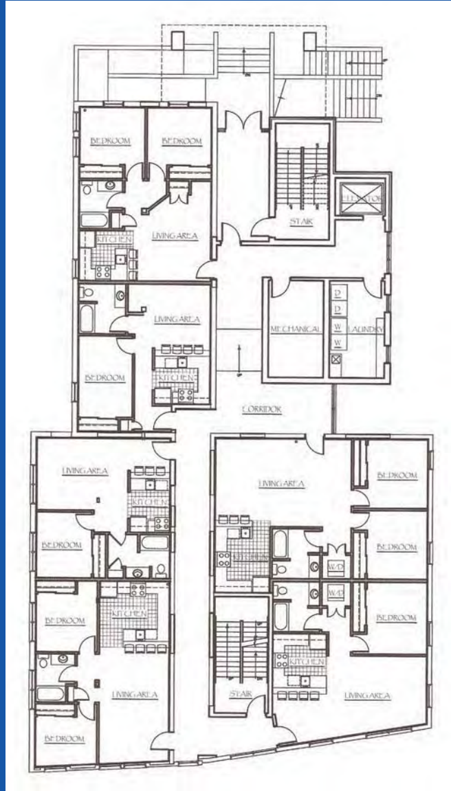
Second & Third Floor Plan (Residential)
